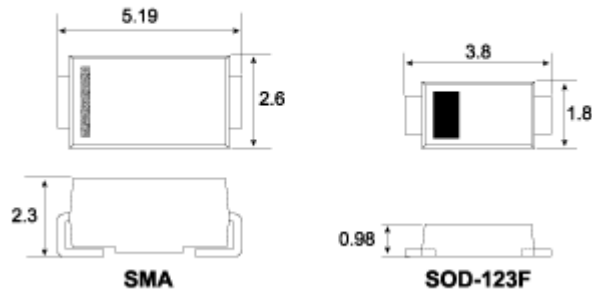
Comparison of SOD-123F to SMA (Dimension in mm)
